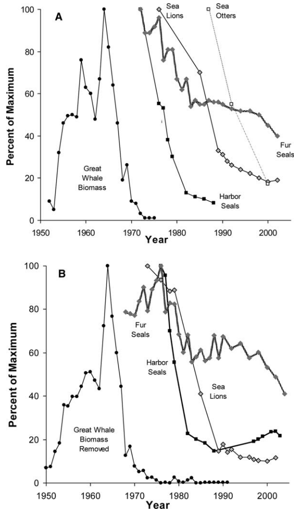
Fig. 1. Biomass of large whales removed and changes in abundance of harbor seals, Steller sea lions, northern fur seals and northern sea otters at select sites in the Gulf of Alaska and Aleutian Islands. Panel A shows the data compiled by Springer et al. (2003) to conclude that declines of pinnipeds were sequential. Panel B shows harbor seal counts from the southwest beach of Tugidak Island, non pup Steller sea lion counts from the nearby Chowiet Island, and northern fur seal pup counts from St. Paul Island. These data suggest that all three populations began declining at about the same time. The biomass of large whales removed shown in Panel B is the annual catch in the Bering Sea, Aleutian Islands and Gulf of Alaska (i.e., catches from 50° N latitude and above) (from Mizroch and Rice, 2006) and differs from that calculated by Springer et al. in Panel A. Note that catch is not an index of numbers or biomass of whales present. See text for further details.
