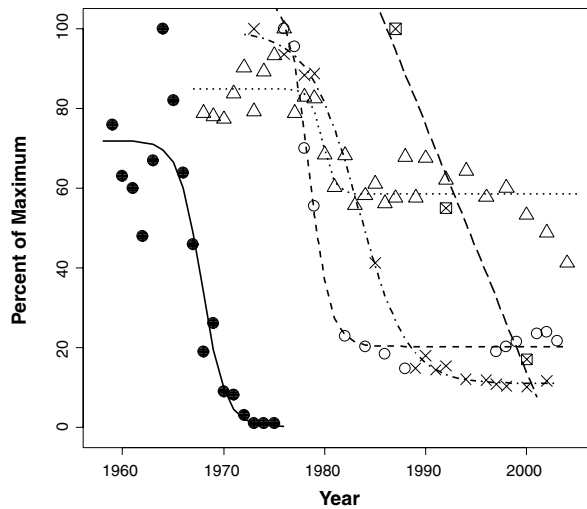
Fig. A.1. Model fits to all species and whale catch data. Solid line and solid circles are whale catch data, short dashed line and open circles are harbor seal data, dotted line and triangles are for northern fur seal data, dash-dot line and x's are Steller sea lion data, and the long dashed line and squares filled with x's are for sea otter data.
